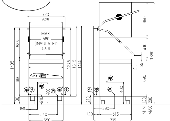
HOOD 800 - HOOD 110 HOOD 110-T - HOOD 110-TT
